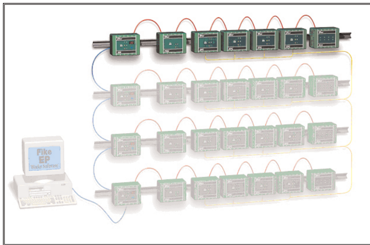
Figure 2: Multi-Loop Schematic Representation of EPACO Bus Network
